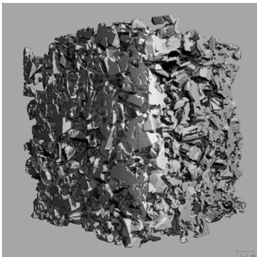
Figure 3: A three-dimensional reconstruction of a sample after being subjected to a large temperature gradient for five days.
